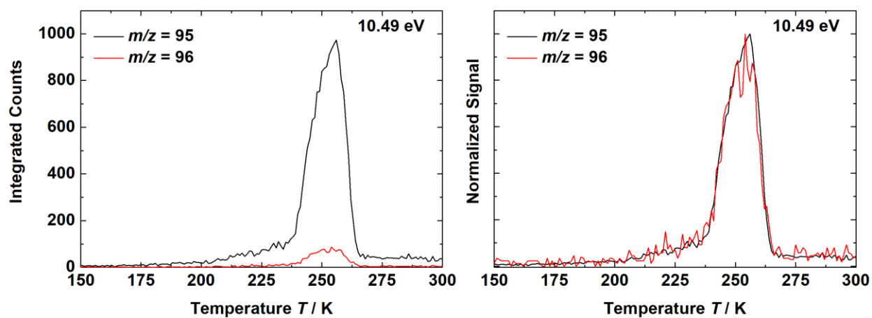
Figure S7. Temperature Programmed Desorption profiles of protonated (black lines) and deuterated (red lines) acetaldehyde dimers forming in the irradiated acetaldehyde-2,2,2-d 3 ice.
