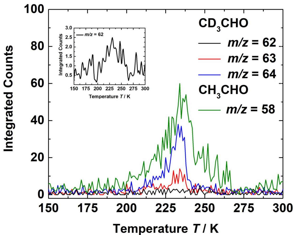
Figure S8. PI-ReToF sublimation profiles of m/z = 62 , 63, and 64 after electron irradiation of acetaldehyde-2,2,2- \text{d}_3 , and m/z = 58 after electron irradiation of acetaldehyde. The inset shows a zoom into smoothed data of the m/z = 62 TPD profile. Spectra were recorded at a photon energy of 10.49 eV.
